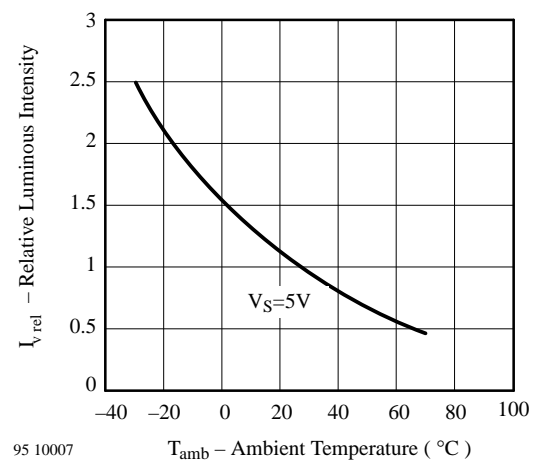
Figure 12. Relative Luminous Intensity vs. Amb. Temperature
