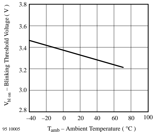
Figure 6. Blinking Threshold Voltage vs. Amb. Temperature
